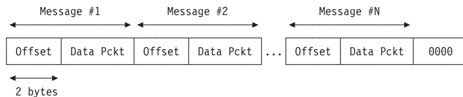
Figure 103. PCCA Block Structure
