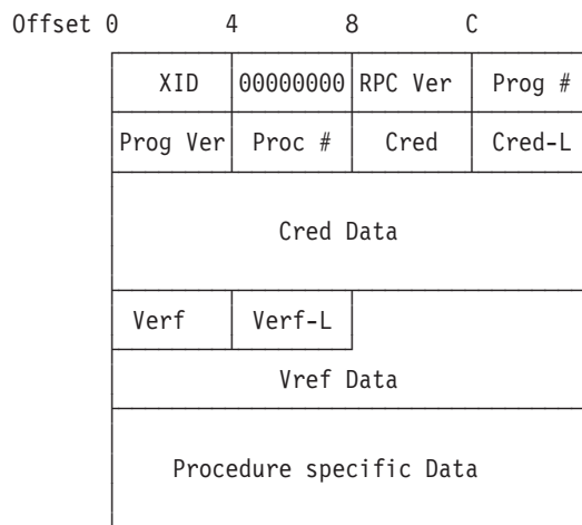
Figure 86. RPC Call Message Structure
