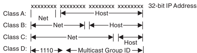
Figure 12. Classes of IP Addresses
