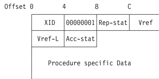
Figure 87. Structure of an RPC Accepted Reply Message
