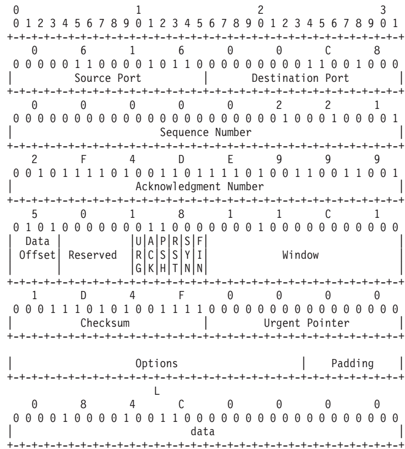
Figure 112. TCP Header Format
