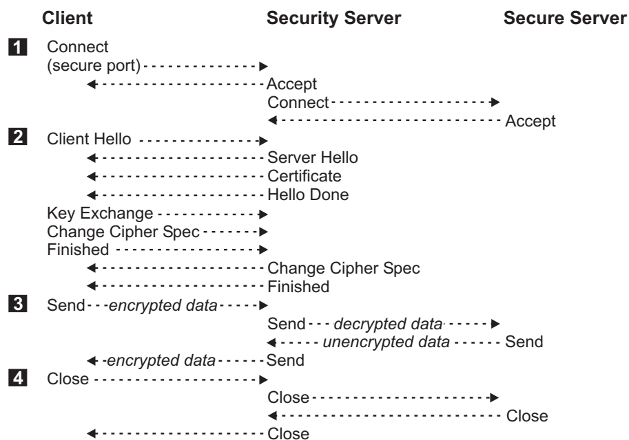
Figure 93. SSL processing flow
