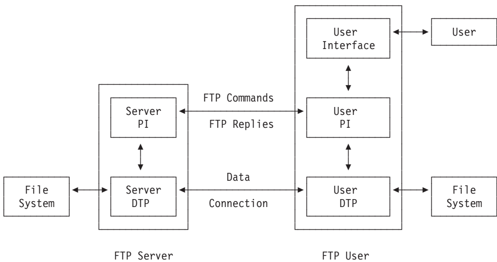
Figure 73. The FTP Model
