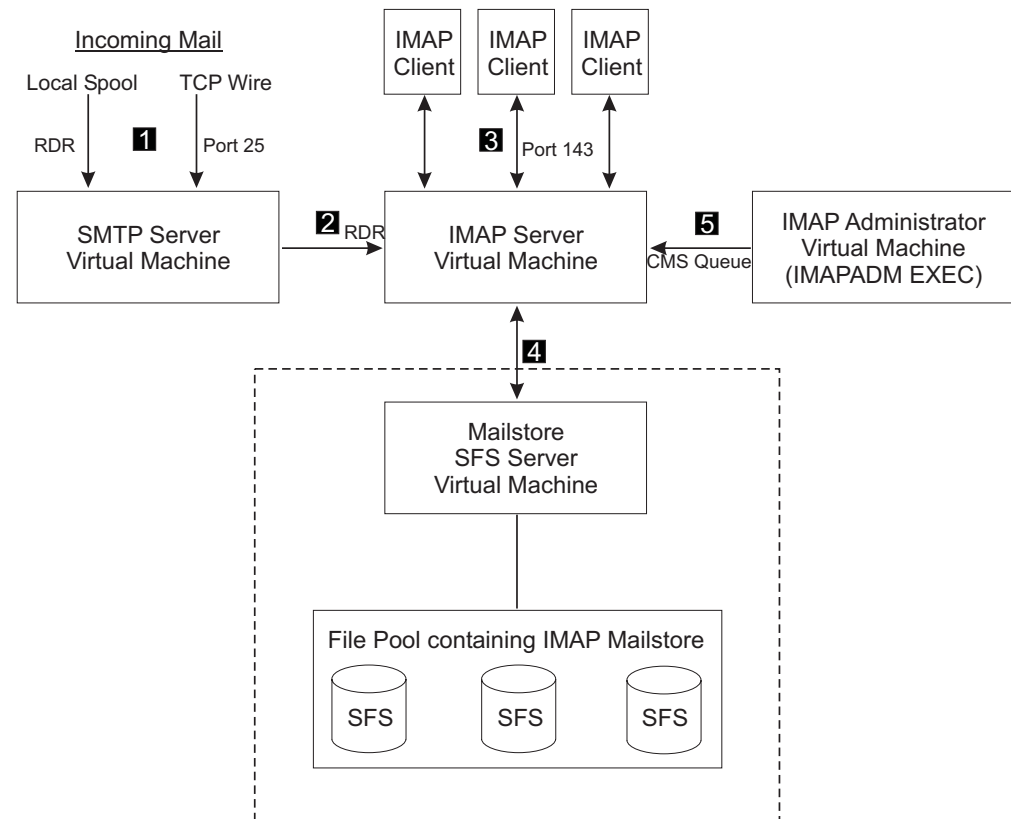
Figure 78. IMAP Client and Server Environment
